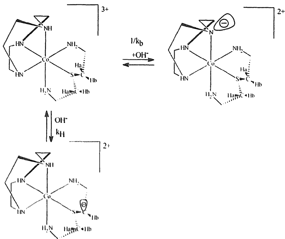
Deprotonation of [\text{Co}(\text{tacn})(\text{daes})]^{3+}
