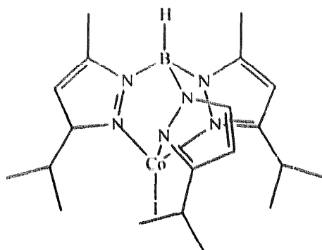
[Hydridotris(3-isopropyl-5-methylpyrazolyl)borato]iodocobalt(II)
