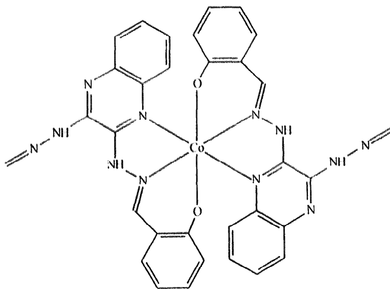
The H 2 BDHQ Cobalt(II) Complex
